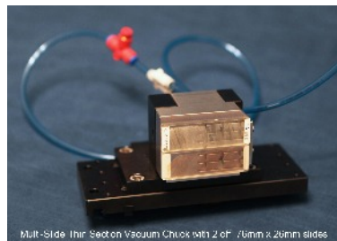
Multi-Slide Thin-section Vacuum Chuck with 2 of 67mm x 26mm slides
