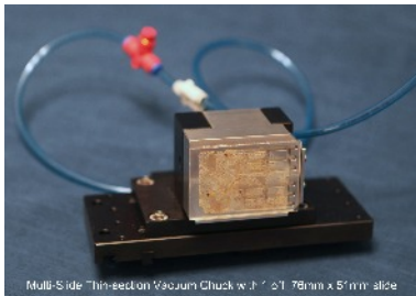
Multi-Slide Thin-section Vacuum Chuck with 76mm x 51mm slide
