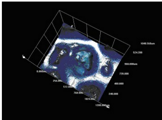
P60g Zirconia - LSCM
